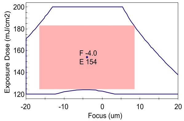
(b) Nominal CD 29.5 microns
