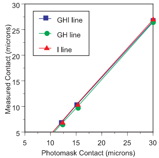
(b) Exposure Wavelength PEB = 100°C
