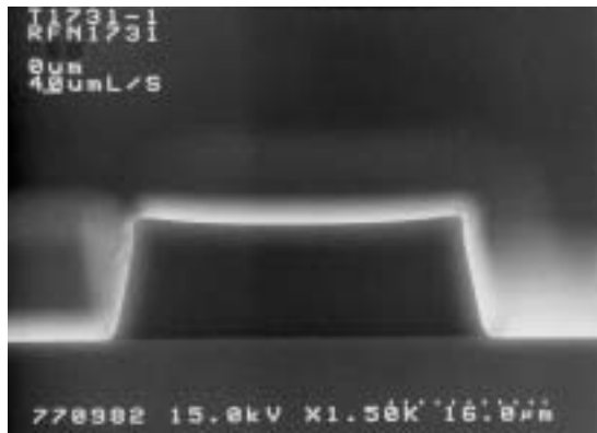
(a) 40 µm line/space
